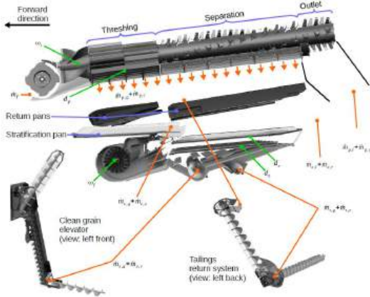
Fig. 1. Threshing, separation and cleaning system material flows.
